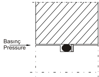
O-ring montajı destek ringi 1 adet O-ring installed with 1 back-up ring
