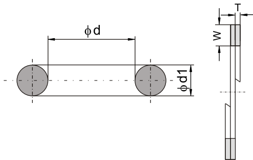
Destek ringi spiral Back-up ring spiral
