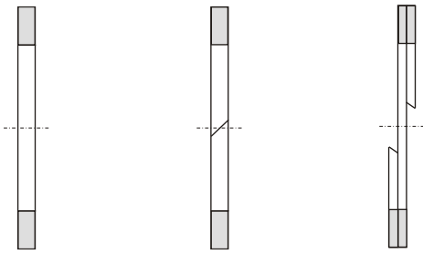
Destek ringi yekpare Back-up ring uncut
