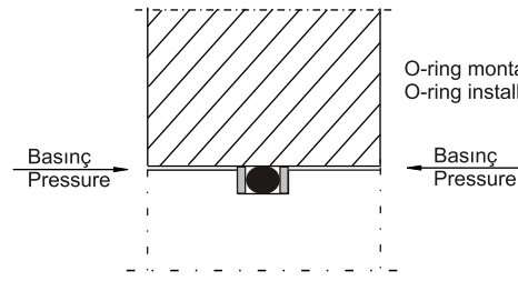
O-ring montajı destek ringi yok O-ring installed without back-up ring
