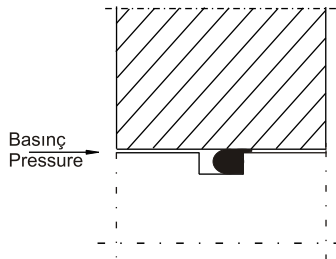
O-ring montajı destek ringi yok O-ring installed without back-up ring
